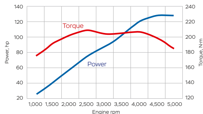
FULL-LOAD CURVE
