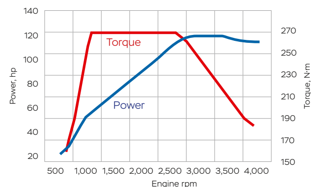
FULL-LOAD CURVE
